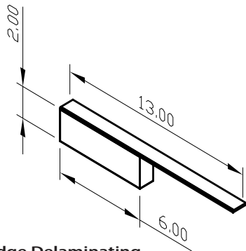
Figure 8 - Edge Delaminating Test Specimen
