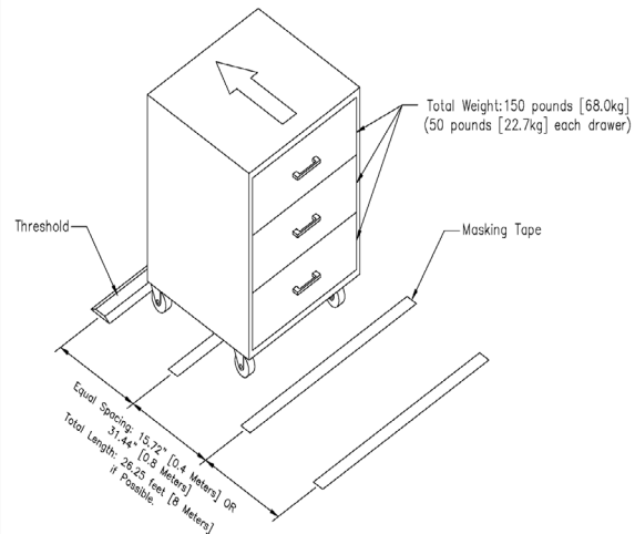
Figure 4. Rolling Stability Test Configuration
