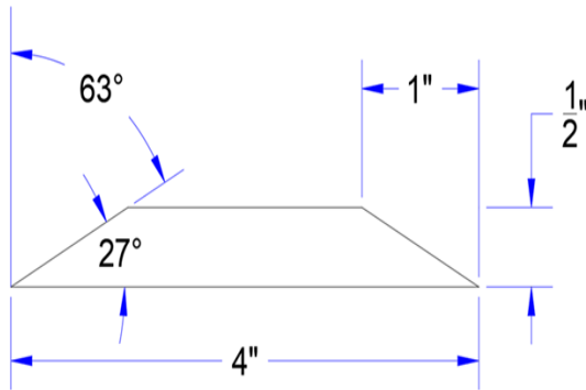
Fig. 1 - Description of Base Cabinet
