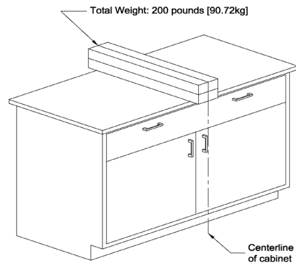
Figure 3. Base Cabinet Concentrated Load Test
