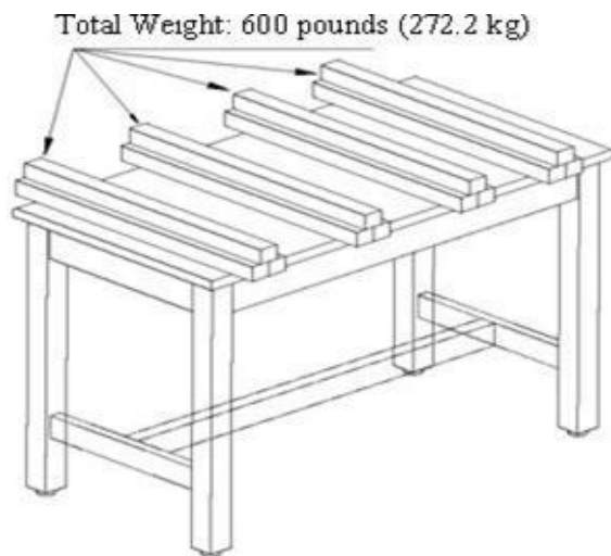
Fig 14 Table Static Load Test Configuration
