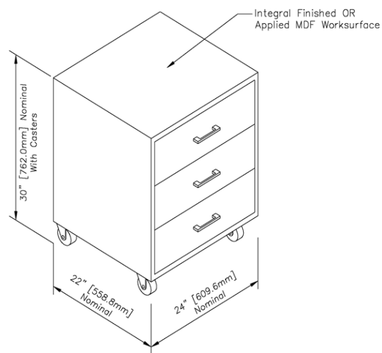
Figure 1. Description of Test Mobile Base Cabinet
