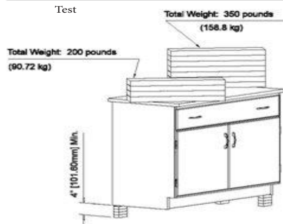
Fig. 4 - Cabinet Torsion
