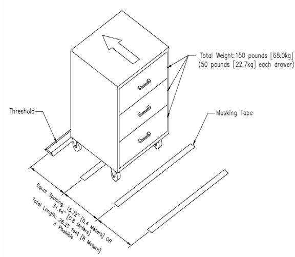
Figure 4. Rolling Stability Test Configuration
