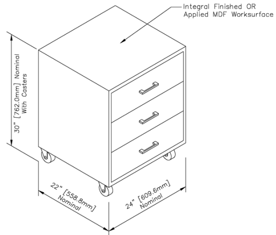
Figure 1. Description of Test Mobile Base Cabinet
