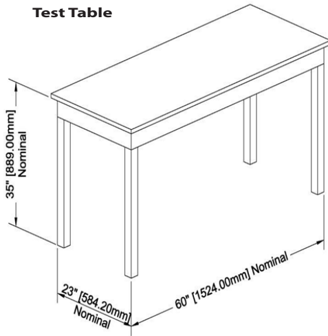
Fig. 10 - Description of Test Table
