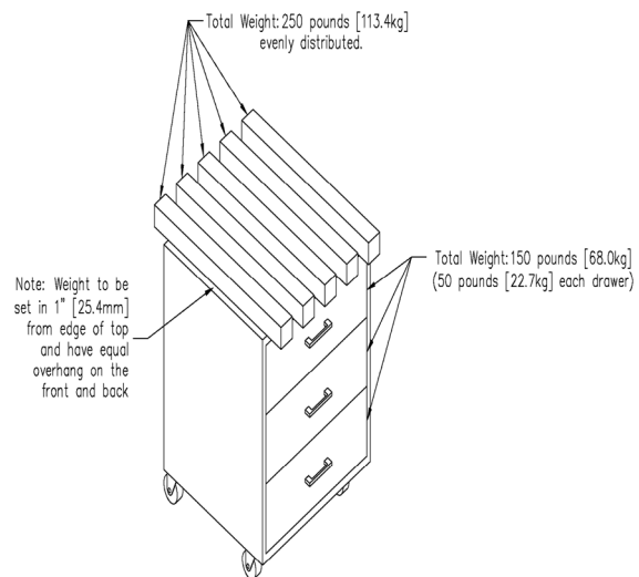
Figure 3. Static Load Test Configuration
