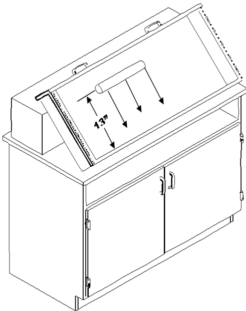
Fig. 7 - Base Cabinet Drawer Internal Rolling Impact Test Configuration
